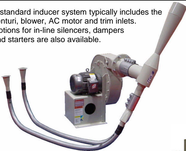
JTW inducer trim conveying systems can be integrated with in-line trim recycling, repelletizing or compacting systems, as shown.
